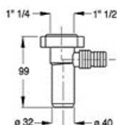
Art. P11/2X230
